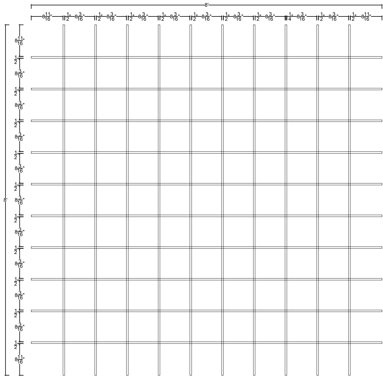
1 PLAN
