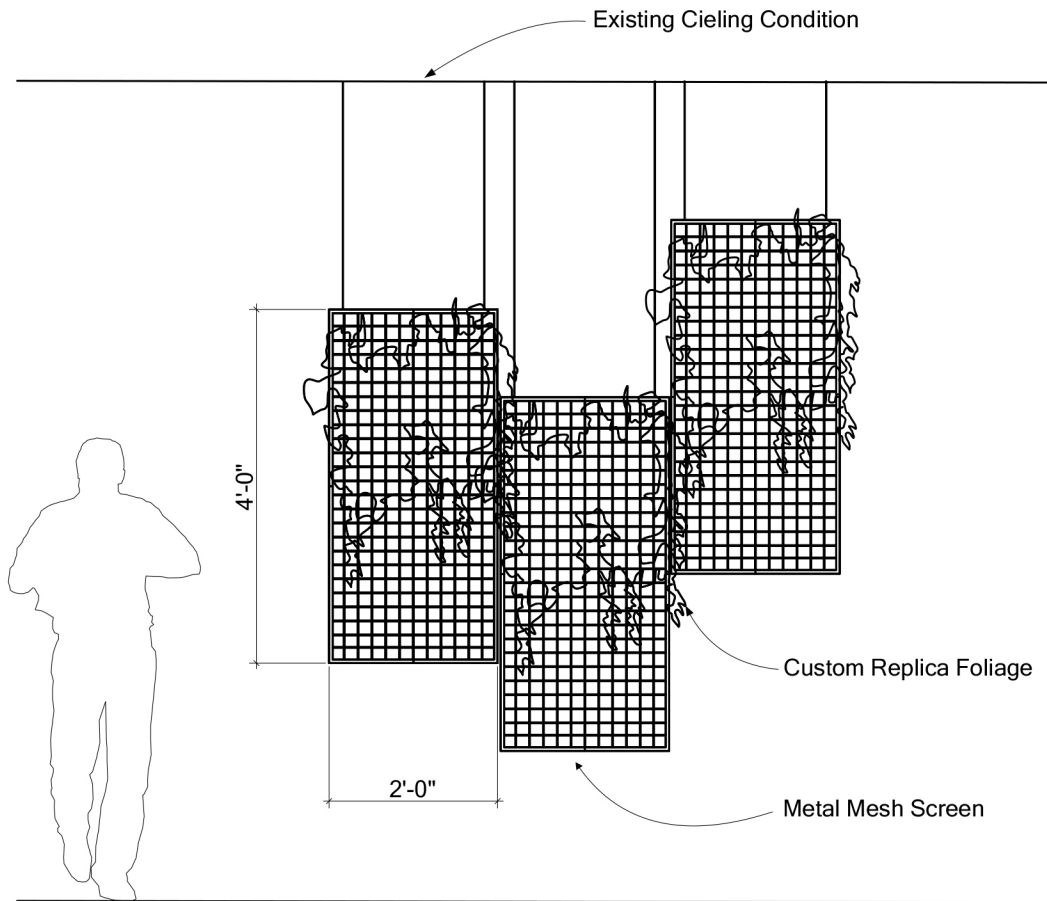
1 FRONT VIEW
