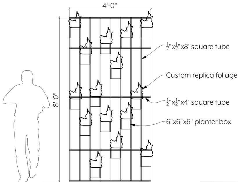
1 FRONT VIEW
