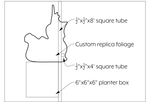
4 DETAIL A.1
