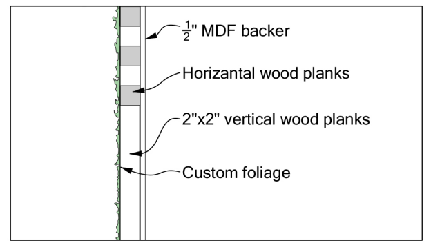
② DETAIL A.1
