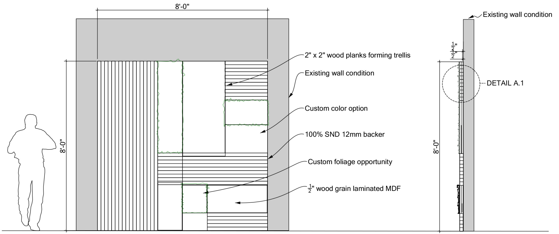
① FRONT VIEW
