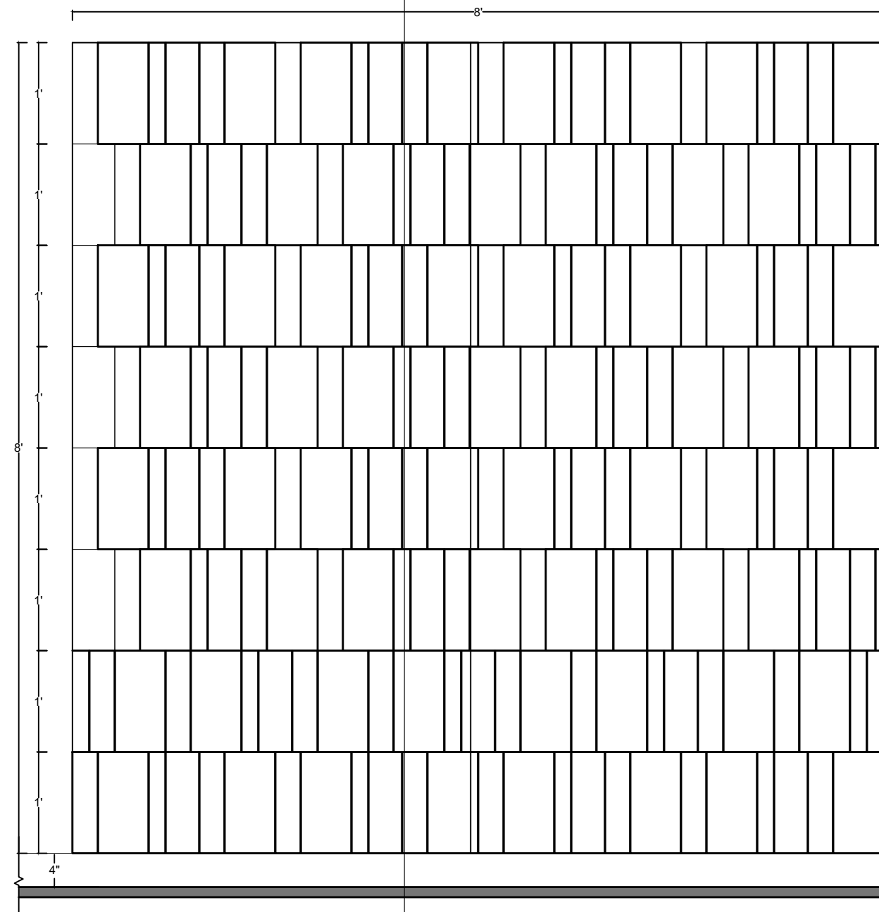
4 ELEVATION ALEXANDRIA-8#PFCALX2403 Scale: 3/4" = 1'-0"
