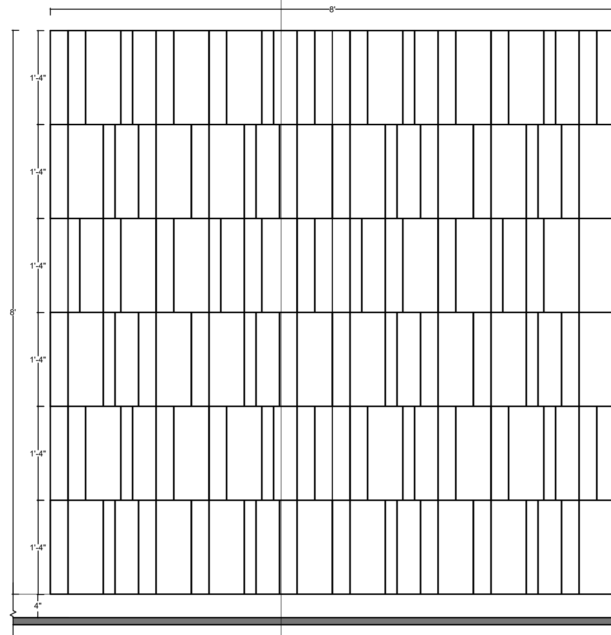
4 ELEVATION ALEXANDRIA-6#PFCALX2402 Scale: 3/4" = 1'-0"
