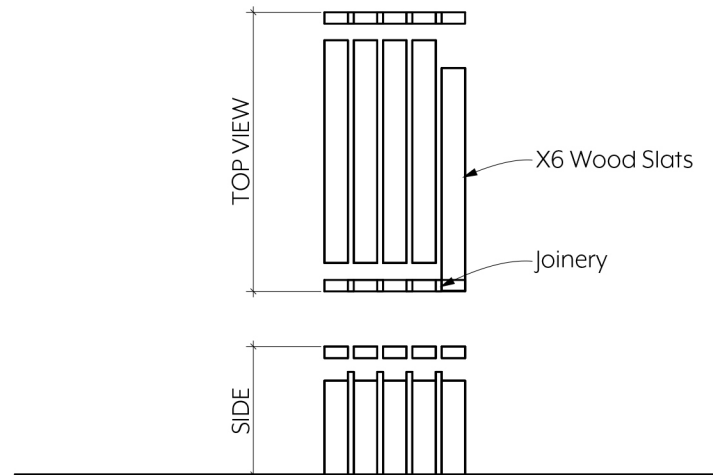
1 A-2 DETAIL VIEW
