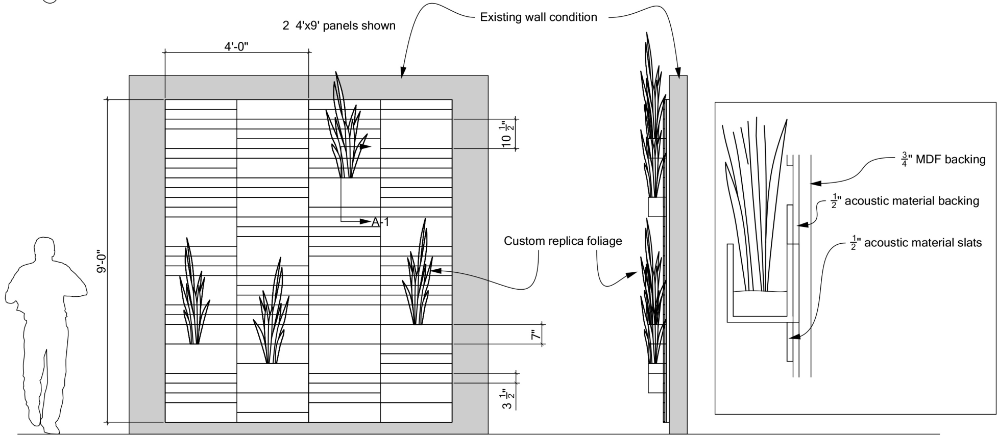
3 TOP VIEW
