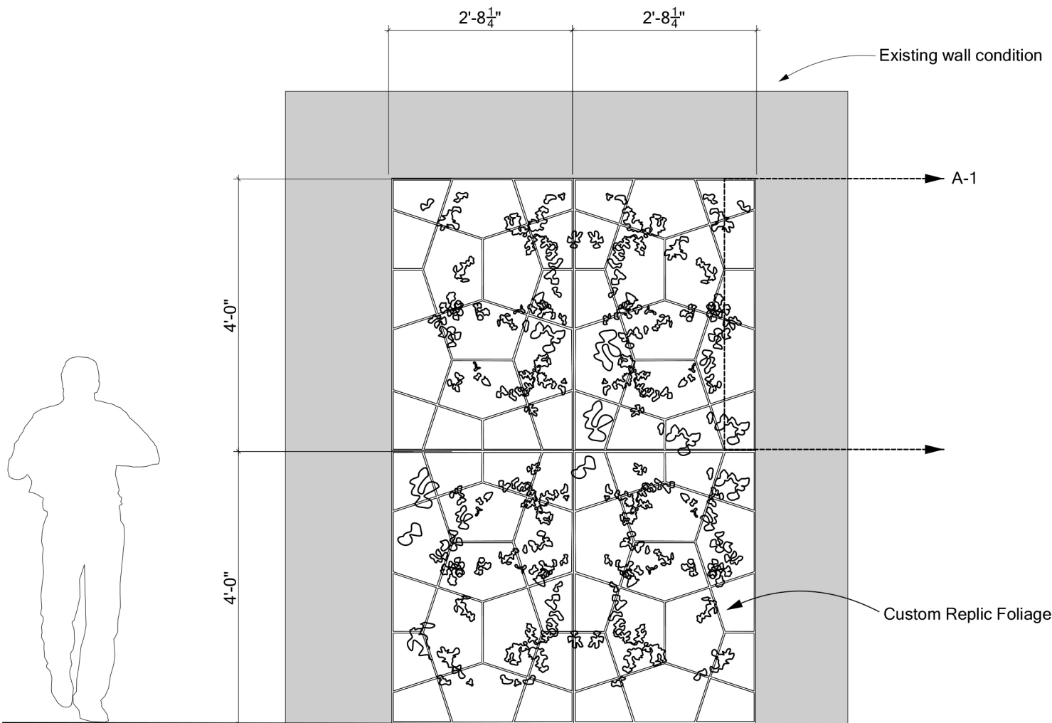
① FRONT VIEW
