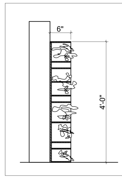
② A-1 SECTION VIEW
