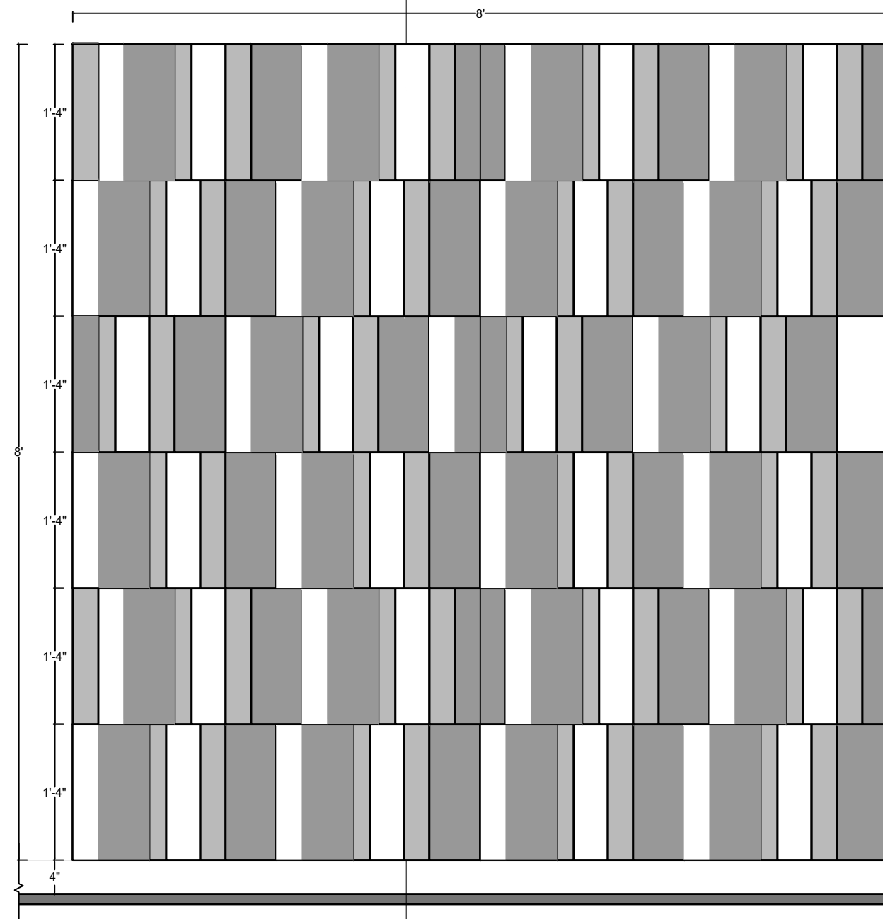
④ ELEVATION BOOKCASE-6#PFCALX2402 Scale: 3/4" = 1'-0"
