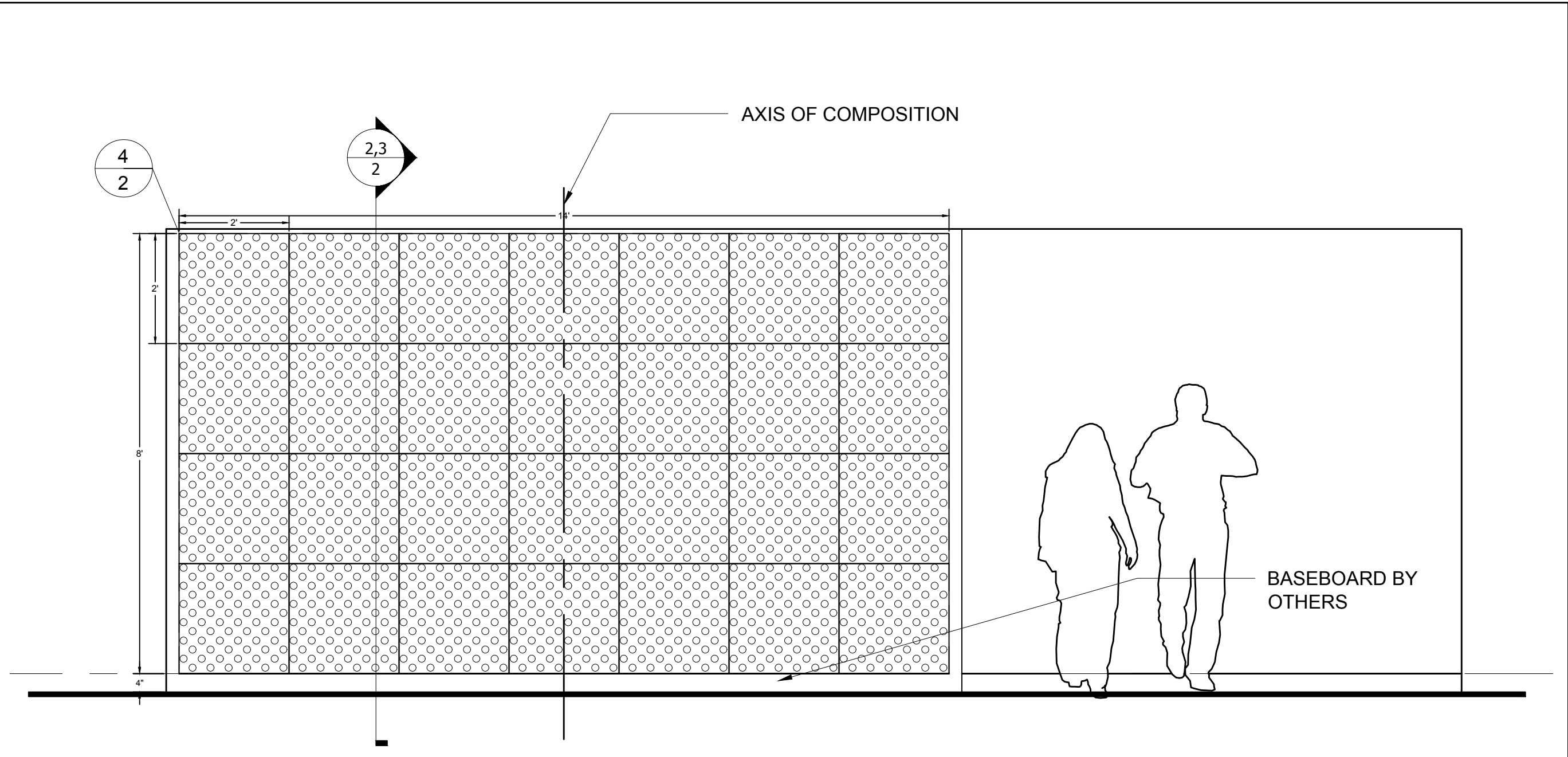
1 MODULAR ELEVATION DESIGN
