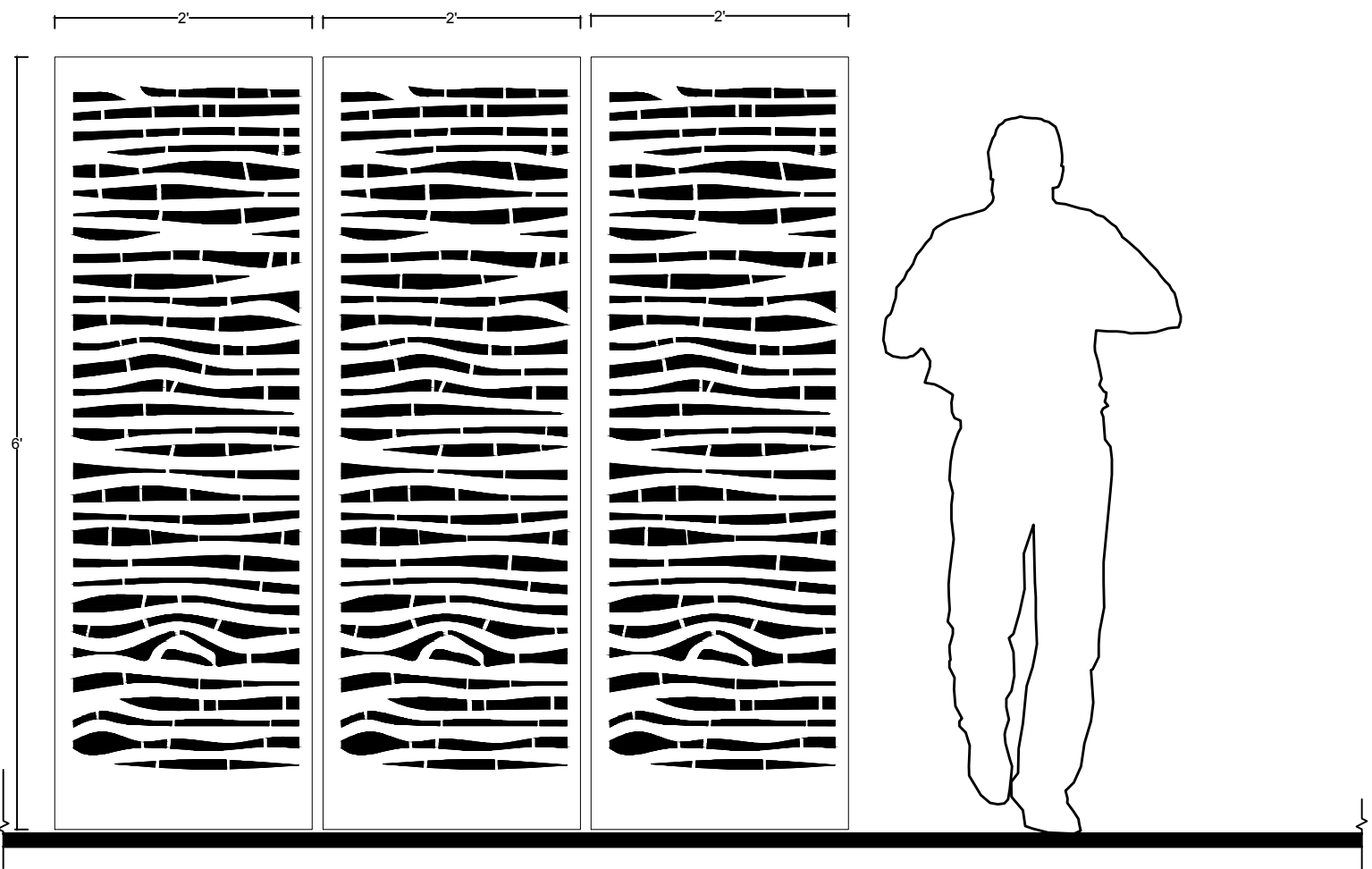
4 ELEVATION BUFFER COMPONENTS Scale: 3/4" = 1'-0"
