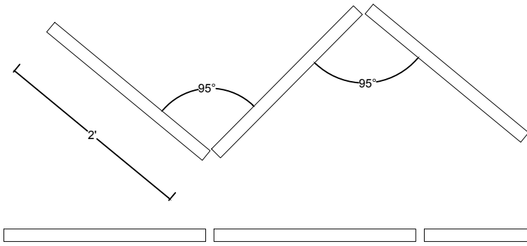
2 PLAN VIEW BYOBU Scale: 3/4" = 1'-0"
