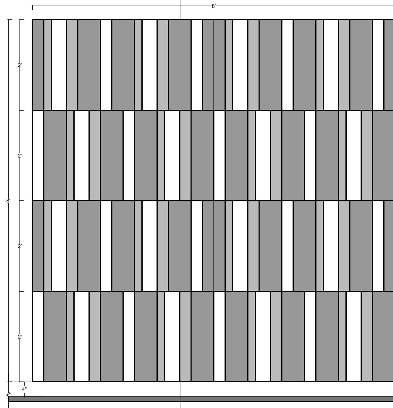
4 ELEVATION BOOKCASE-4#SCCBOK201 Scale: 3/4" = 1'-0"
